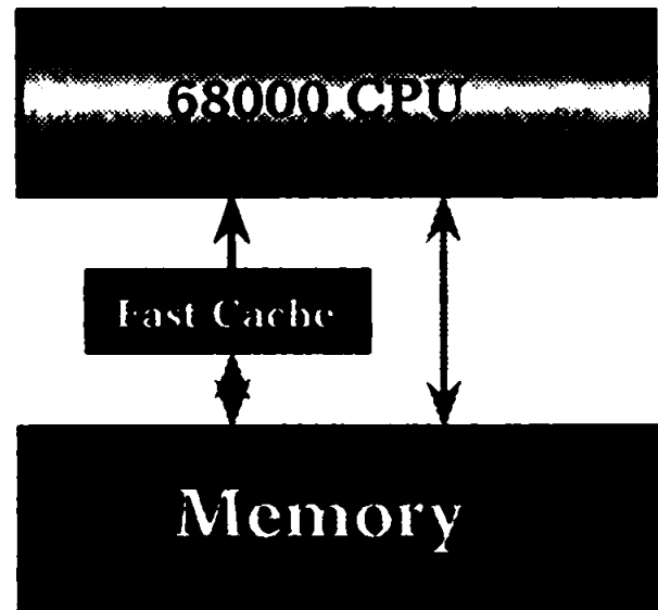
Illumination 12 - Load the next instruction from Cache, not Memory
