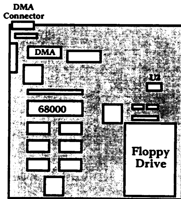
Illumination 28 - Location of U2 and DMA Connector
