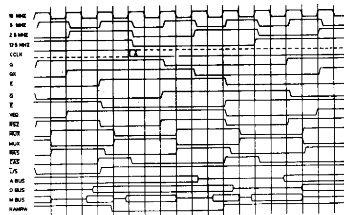
FIGURE 3-1 CLOCK TIMING
