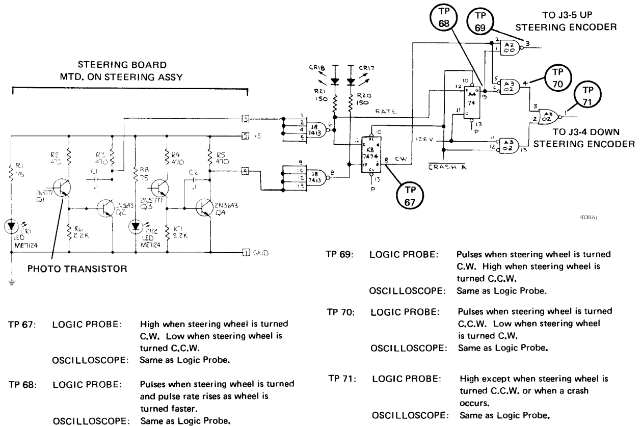
Figure 2-18. Steering Control
