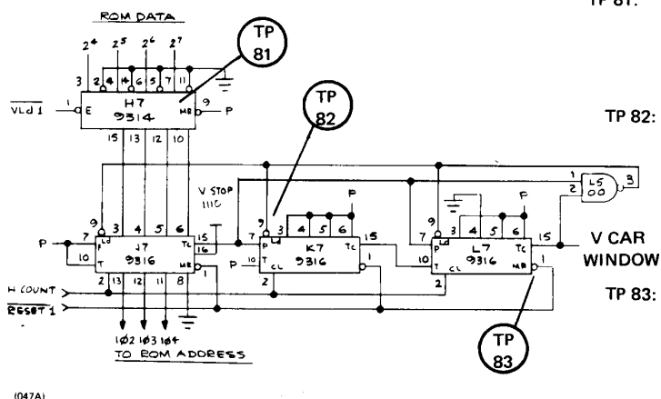
Figure 2-26. Vertical Car Motion
