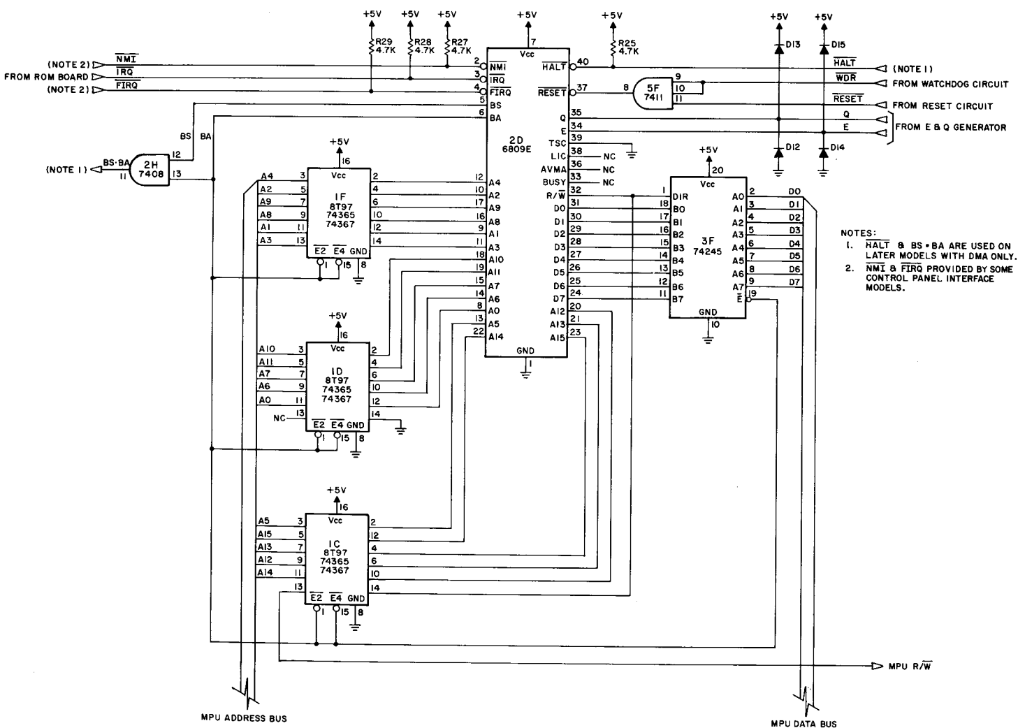
Figure 3-3. MPU
