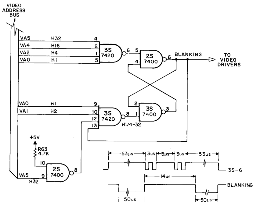
Figure 3-14. Blanking Circuit
